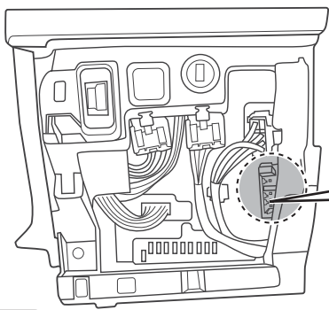
fuse holder
